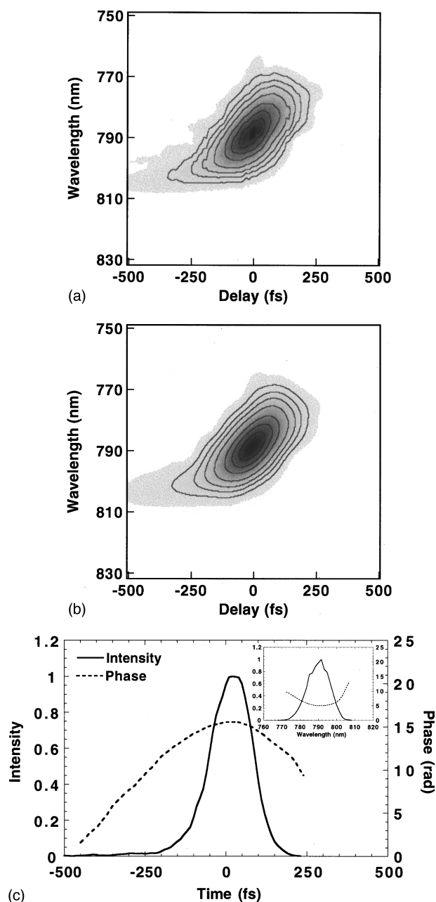
FIG. 4. (a) Experimental multishot FROG trace for an ultrashort laser pulse with positive linear chirp. (b) FROG trace for the pulse retrieved by the algorithm. (c) Retrieved intensity and phase. Note the similar pulse intensity and phase to that shown in Fig. 2 for a linearly chirped pulse. In Figs. 4 and 5, contour lines represent the values: 2%, 5%, 10%, 20%, 40%, 60%, and 80%.
